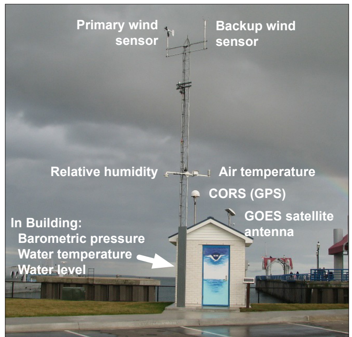
Mackinaw City, MI water level station. Typical water, meteorological, and GPS sensor configuration. Photo: Jeff Oyler, NOS.
