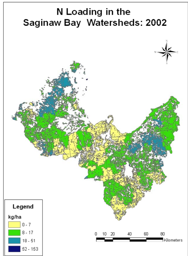
Fig. 3 Distribution of nitrogen (N) from animal manure (kg/ha) by zip code in the Saginaw Bay Basin (data source: www.census.gov).
