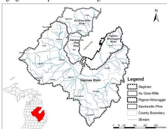
Fig. 1 Boundary of the Saginaw Bay Basin
