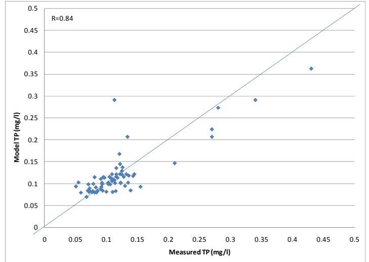
Fig. 4 Model calibration results for TP concentration at Essexville, MI.
