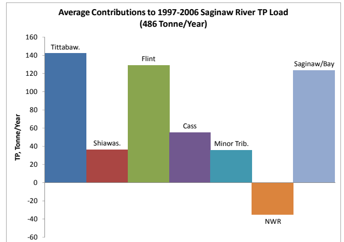
Fig. 5 TP annual loads for different parts of the Saginaw River Basin.
