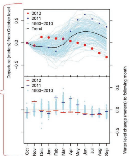
FIG. 1. Satellite image of (left) the North American Laurentian Great Lakes and (right) seasonal patterns in monthly average Lake Erie water levels. Data from 1918 to 2012 are based on a network of gauges around Lake Erie, and data from 1860 to 1917 (before a network was established) are based on a “master gauge.” (Image: NASA and NOAA CoastWatch)
