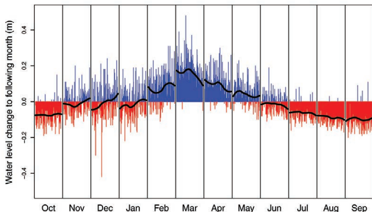
FIG. 2. Month-to-month changes in Lake Erie monthly average water levels. Vertical bars in each panel (one panel for each month) represent the water-level change (m) from the month indicated at the bottom of the panel to the following month for each year from 1860 to 2012. The left-most panel, for example, includes water-level changes from Oct to Nov. Blue vertical bars indicate an increase in monthly water level; red vertical bars indicate a decrease in monthly water level. The black line within each panel indicates the long-term trend.
